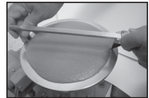
Flow Table
